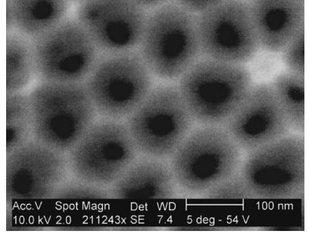
FIG. 1. SEM image of the top surface of a porous alumina sample [30].
